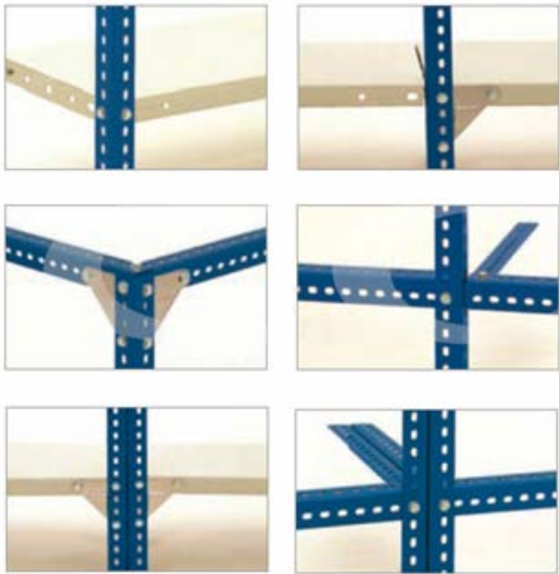
Slotted Angle and Shelves Assembly
