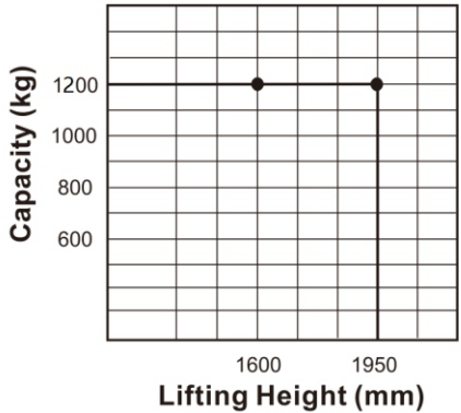
Load chart
