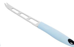
KWKTC008 Thickness: 1.2mm Length: 255mm
